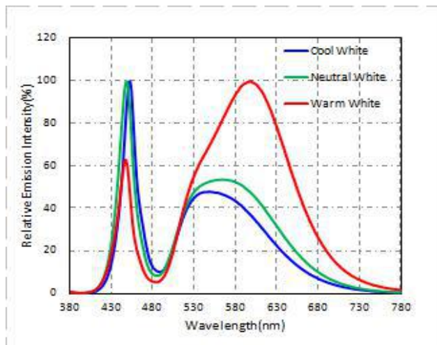
Fig 1. Color Spectrum, T_j = 25^\circ\text{C} R_a \geq 90
