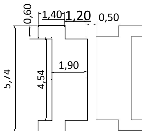
Soldering patterns
