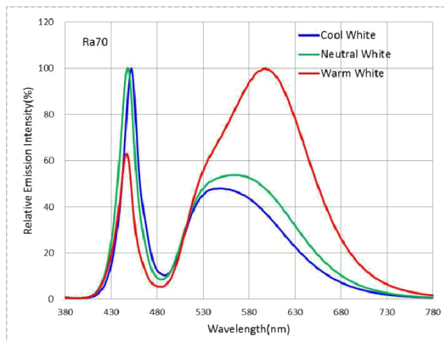
Fig 1. Color Spectrum, T_j = 25^\circ\text{C}
