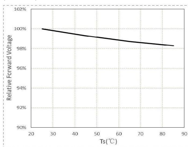
Fig 6. Surface Temperature vs. Relative Forward Voltage (IF=65mA)
