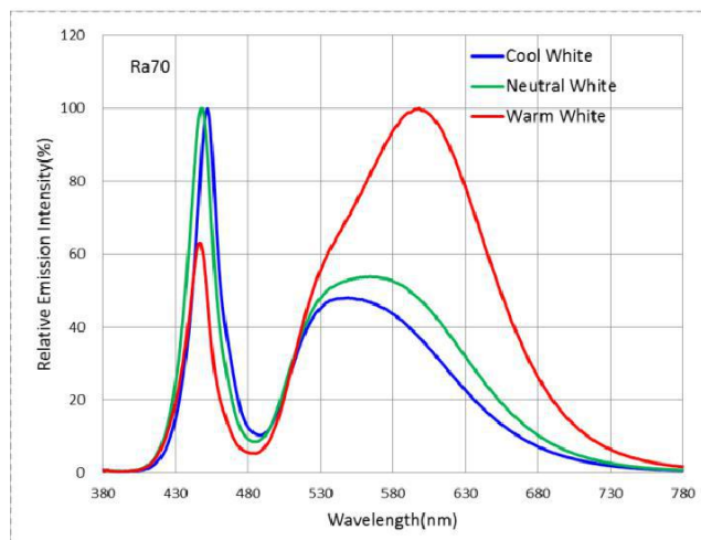
Fig 1. Color Spectrum, Ta = 25°C
