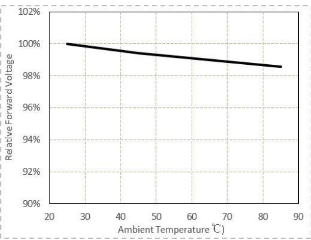
Fig 6. Ambient Temperature vs. Relative Forward Voltage (IF=65mA)
