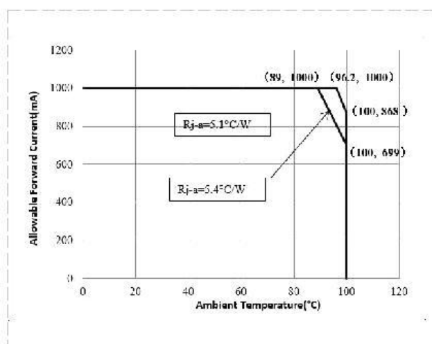
Fig8 . Ambient Temperature vs.Maximum Forward
