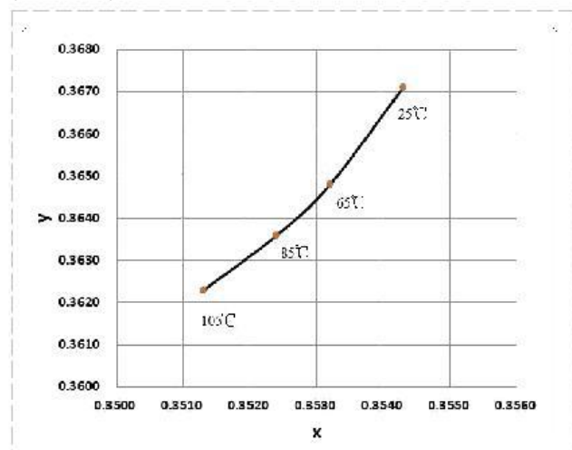
Fig 7. Ambient Temperature vs. CIE(x,y)
