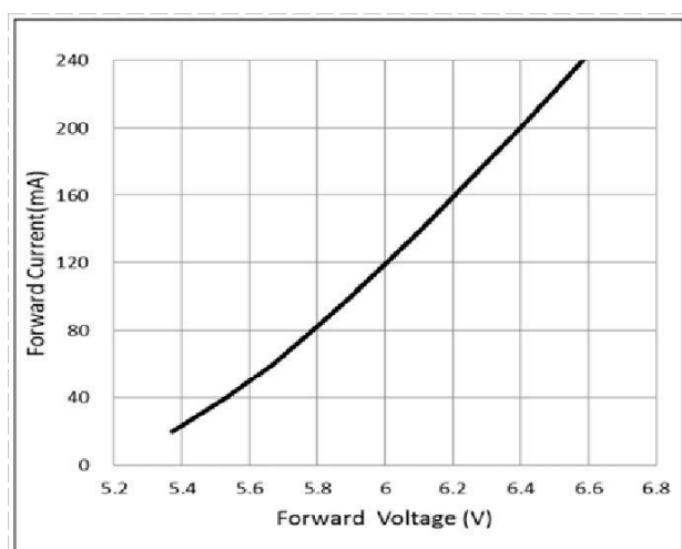
Fig . Forward Current vs. Forward Voltage, T_j = 25
