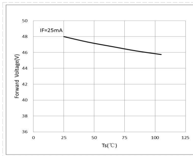
Fig 6. Ambient Temperature vs. Relative Forward Voltage ( I_F=25\text{mA} )
