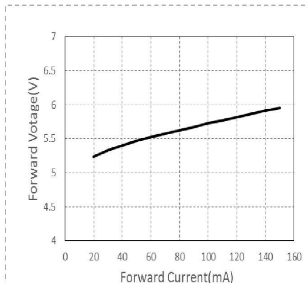
Fig 4. Forward Current vs. Forward Voltage, T_j = 25^\circ\text{C}
