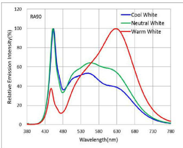
Fig 5. IF--- Relative Luminous
