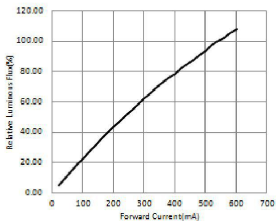
Fig 5. IF--- Relative Luminous
