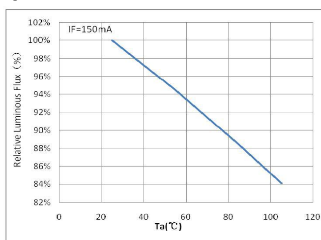
Fig 5. Ta—Relative Luminous flux, Ta = 25°C
