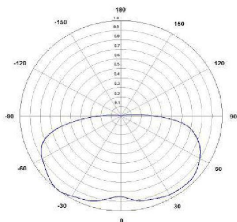
Fig 2. Viewing Angle Distribution, Ta = 25°C
