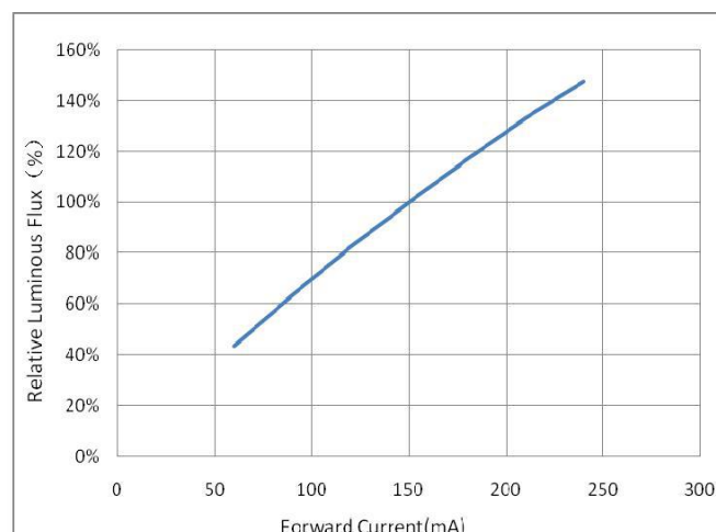
Fig 3. .IF--- Relative Luminous flux, Ta = 25°C
