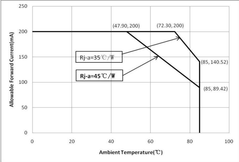
Fig 8, Maximum Forward Current vs. Ambient Temperature
